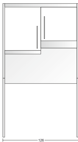
SLDH 120 - H2220
